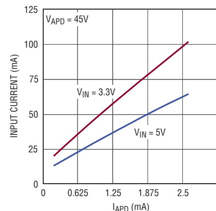
Input Current vs APD Current
